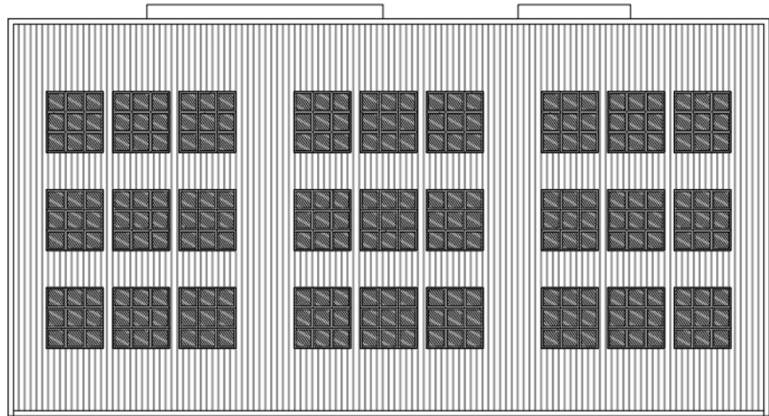
ROOF PLAN
